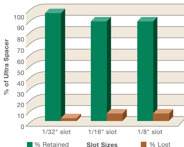
Figure 1. Slot Test Chart
